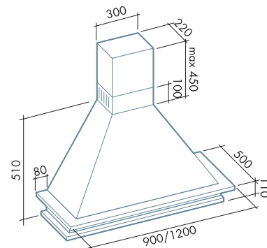
parete/wall
